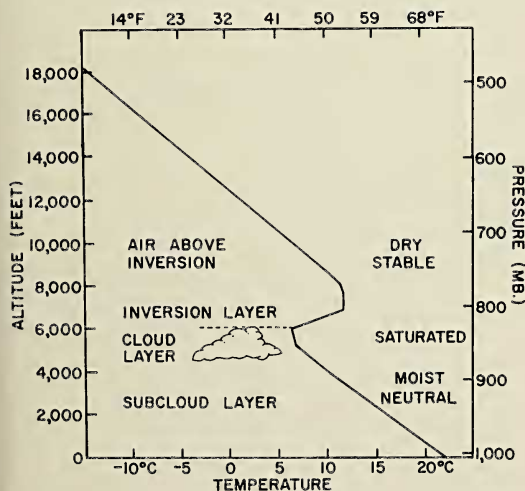
FIG. 2. Structure of the trades in Hawaii.
